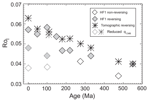
Fig. 10. Local Rossby number versus age from HF1 and tomographic dynamos. Symbols with dashed lines denote reduced CMB heat flow dynamos; unshaded symbols denote non-reversing dynamos.
