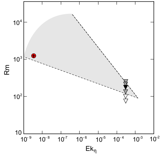
Fig. 3. Magnetic Reynolds number versus magnetic Ekman number for dynamos with present-day mantle structure from Table 4 (triangles) compared with present-day geodynamo (circle). Triangle shades indicate dynamo reversal behavior (shaded = reversing, unshaded = non-reversing, black = present-day reversal rate). Light grey denotes the region of Earth-like dynamo behavior determined by Christensen et al. (2010) with a lower bound corresponding to the power law (36).
