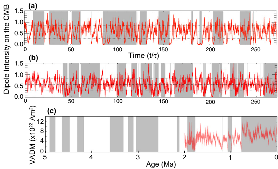
Fig. 5. Comparison of present-day dynamos with paleomagnetic data based on 20 kyr dipole free decay time for the core. (a) Dipole intensity and polarity reversal sequence from the present-day HF1 dynamo. The rms dipole intensity is in dimensionless Elsasser number units; normal and reverse polarity are indicated by shaded and unshaded, respectively. (b) Same for the present-day tomographic dynamo. (c) 0–5 Ma GPTS reversal sequence from Ogg (2012) and 0–2 Ma SINT2000 virtual axial dipole moment (VADM) from Valet et al. (2005).
