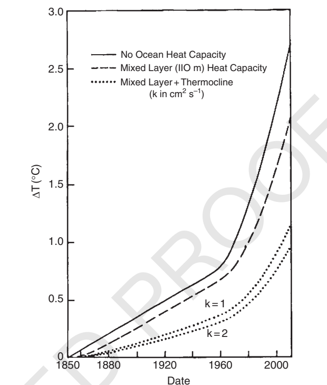
Fig. 18. Global mean warming computed for the \text{CO}_2 and trace gas scenarios in Table 4.
