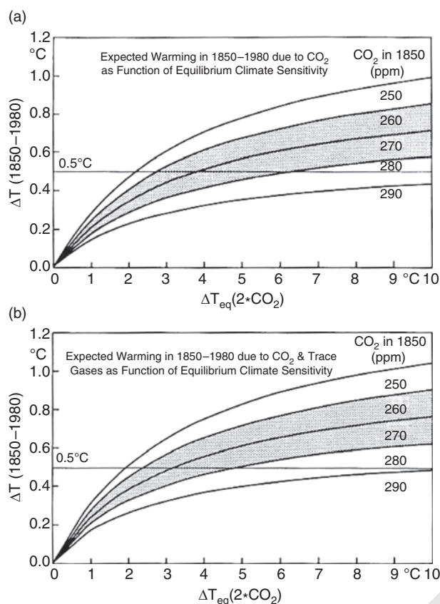
Fig. 17. Computed global warming between 1850 and 1980 as a function of the equilibrium climate sensitivity for doubled \text{CO}_2 (315 ppm \rightarrow 630 ppm), \Delta T_{\text{eq}}(2 \cdot \text{CO}_2) . Results are shown for five values of the assumed abundance of \text{CO}_2 in 1850; the shaded area covers the range 270 \pm 10 ppm recommended by WMO (1983). (a) includes only \text{CO}_2 growth, while (b) also includes the trace gas growths of Table 4. In all cases \text{CO}_2 increases linearly from the 1850 abundance to 315 ppm in 1958 and then according to measurements of Keeling et al. (1982).
