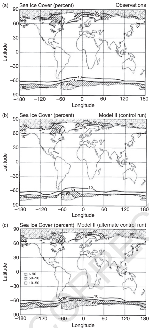
Fig. 2. Annual-mean sea ice cover. (a) observational climatology of Walsh and Johnson (1979) for the northern hemisphere and Alexander and Mobley (1976) for the southern hemisphere. (b) our standard control run of the 3-D climate model. (c) alternate control run, as described in the text.
