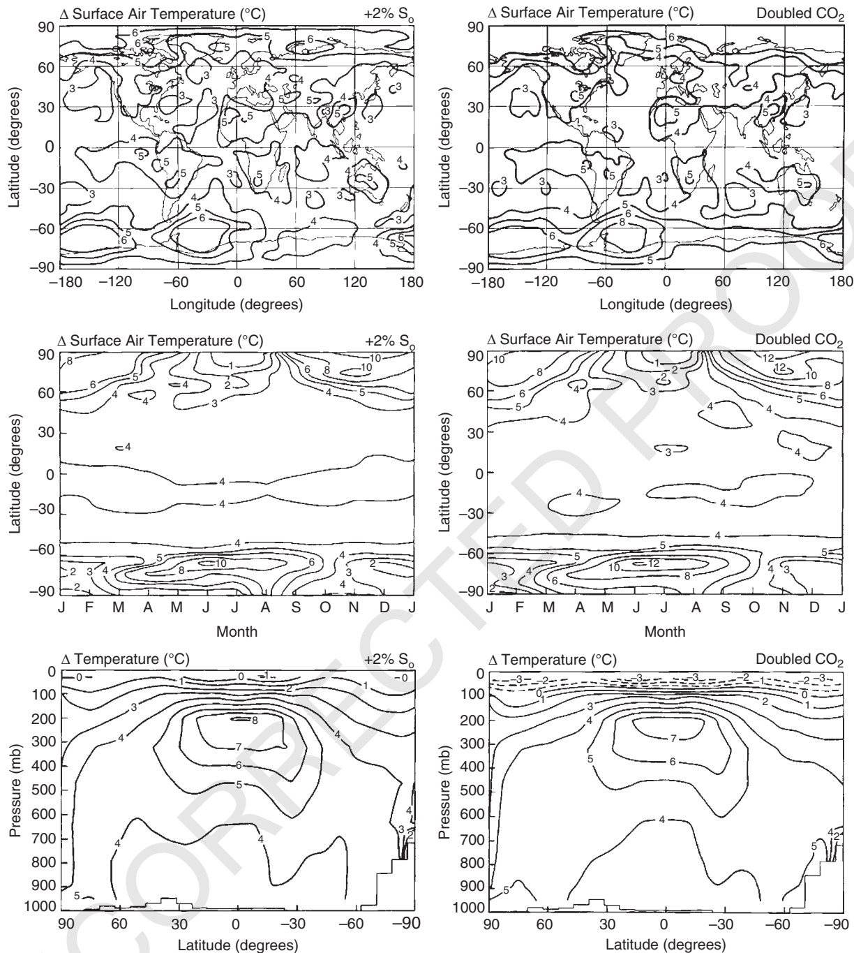
Fig. 4. Air temperature change in the climate model for a two percent increase of solar irradiance (left) and for doubled atmospheric \text{CO}_2 (right). The upper graphs show the geographical distribution of annual mean surface air warming, the middle graphs show the seasonal variation of the surface air warming averaged over longitude, and the lower graphs show the altitude distribution of the temperature change averaged over season and longitude.
