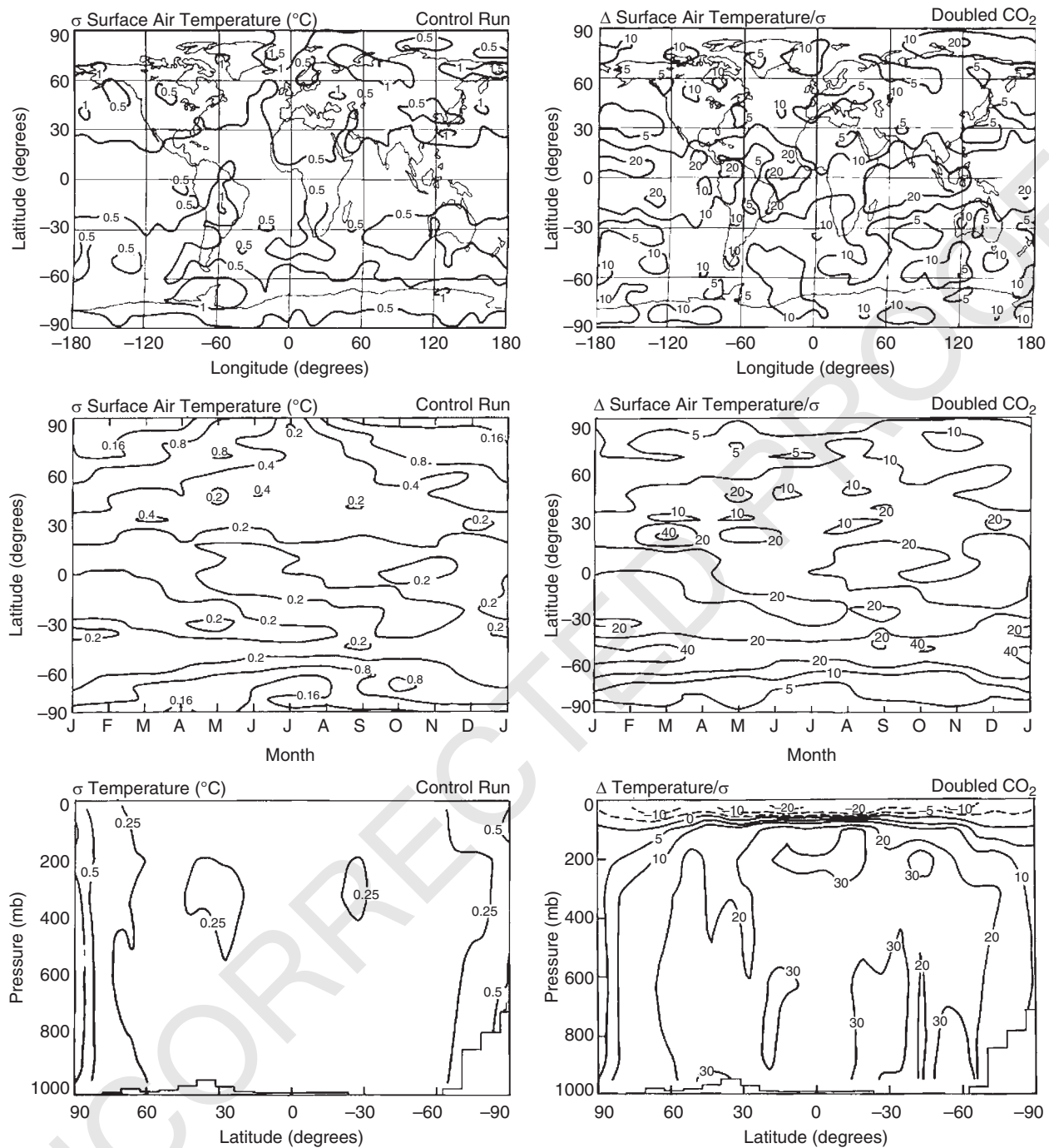
Fig. 5. Left side: standard deviation of temperature for the last 10 years in the control run. Right side: ratio of temperature change for years 26–35 of the doubled \text{CO}_2 experiment to the standard deviation of temperature in the control run.
