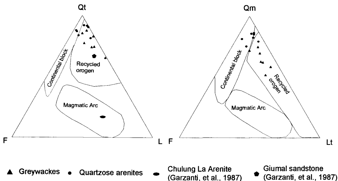
Figure 7. Detrital mode plot of Tianba Flysch. Tectonic fields are from Dickinson and Suczek (1979). Giumal sandstones and Chulung La Arenite from Zanskar (Garzanti et al. 1987) are shown for reference on the QtFL plot.
