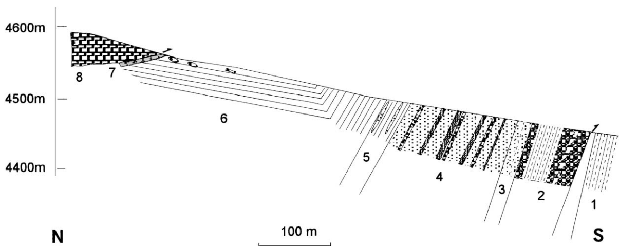
Figure 4. Tianba cross section (section 2; see fig. 3 for location). Unit numbers correspond to those on the stratigraphic column (fig. 5), which includes explanation of the patterns.
