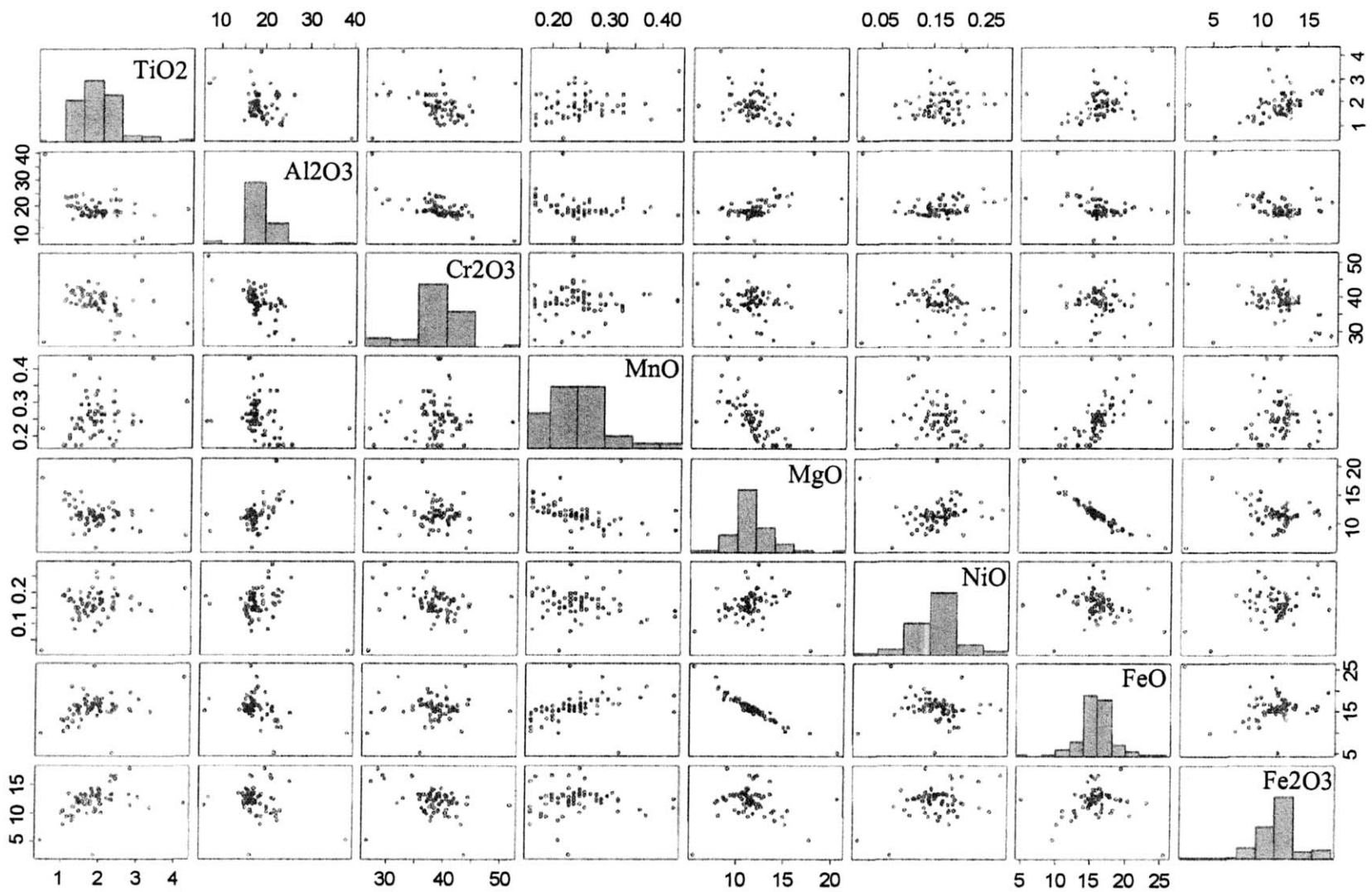
Figure 8. Chemical compositions of detrital Cr-rich spinels using pairs plot from S-Plus
