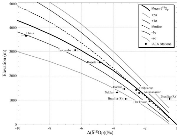
Fig. 4. \Delta(\delta^{18}\text{O}_p) versus elevation of IAEA–GNIP stations versus trajectories of the predicted isotopic composition of precipitation.
