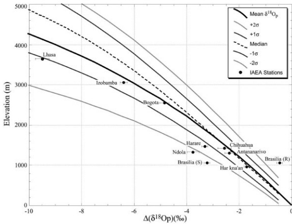
Fig. 4. \Delta(\delta^{18}O_p) versus elevation of IAEA–GNIP stations versus trajectories of the predicted isotopic composition of precipitation.
