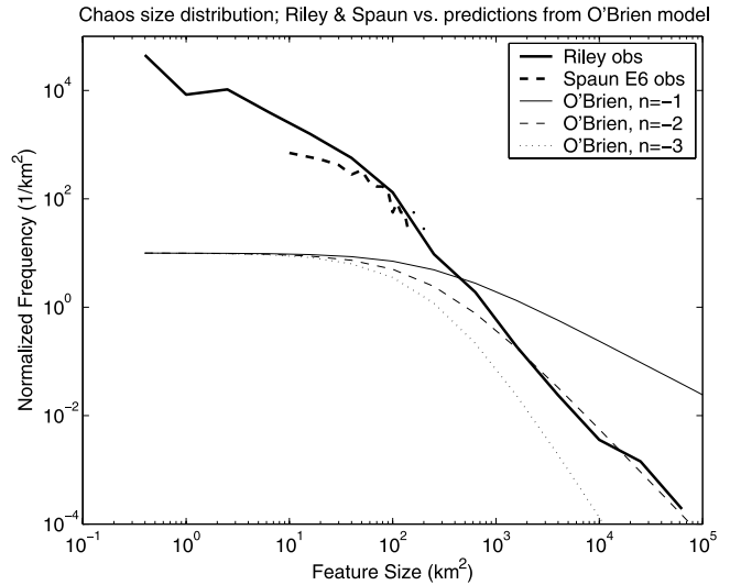
Figure 11. Normalized size distributions for chaos/lenticulae on Europa. Solid thick line: observed distribution from Figure 9b of Riley et al. [2000]. For areas between 100 and 10 5 km 2 , we use Riley's medium-resolution data; for areas <100 km 2 , we use the high-resolution data. Dashed thick line: same, but for Figure 1 of Spaun et al. [2001], E6 orbit data. E11 and E14 data are similar. Thin lines: melt-through size distribution arising from the model of O'Brien et al. [2002], assuming a basal heating scale d_0 = 40 km and a power-law distribution of melt-through event energies with various choices of exponent ( n = -1 , n = -2 , n = -3 ). Y-axis (units 1/km 2 ) represents number of global features per unit size range, not per unit mapped surface area; thus Riley's data imply 130 features on Europa with sizes between 100 and 101 km 2 , 1600 features with sizes between 15 and 16 km 2 , etc.
