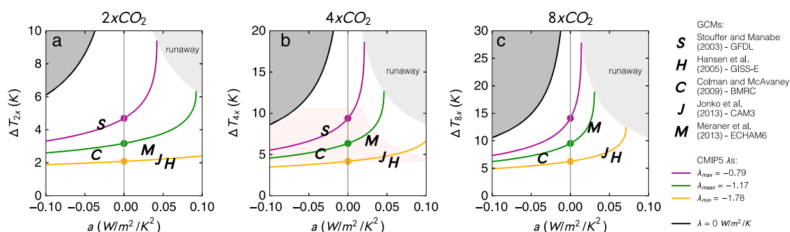
Figure 2. The feedback temperature dependence a versus (a) \Delta T_{2x} , (b) \Delta T_{4x} , and (c) \Delta T_{8x} (the equilibrium warming from one, two, and three doublings of \text{CO}_2 , respectively). Letters represent GCMs and are centered on pairs of a (quadratic estimate, see supporting information, Section S3) and \Delta T_{nx} (reported values). Colored lines show how quadratic estimates of \Delta T_{nx} (using equation (1)) vary with a for fixed values of \lambda , assuming forcings of F_{nx} = \log_2(n)3.71 \text{ W/m}^2 . Colored circles where these lines intersect the center vertical give linear estimates of \Delta T_{nx} . Some lines intersect the shaded regions in the upper right corner of each panel. For values of a greater than these intersections, the quadratic model experiences runaway warming. If we assume that the preindustrial climate was stable, then \lambda \leq 0 , and the dark region in the upper left-hand corner of each panel is inaccessible under the quadratic model. CMIP5 models must lie in the pink region in Figure 2b to avoid quadratic runaway under RCP8.5. Note that the y axis increases proportionally in each panel [Colman and McAvaney, 2009; Hansen et al., 2005; Jonko et al., 2013; Meraner et al., 2013; Stouffer and Manabe, 2003].
