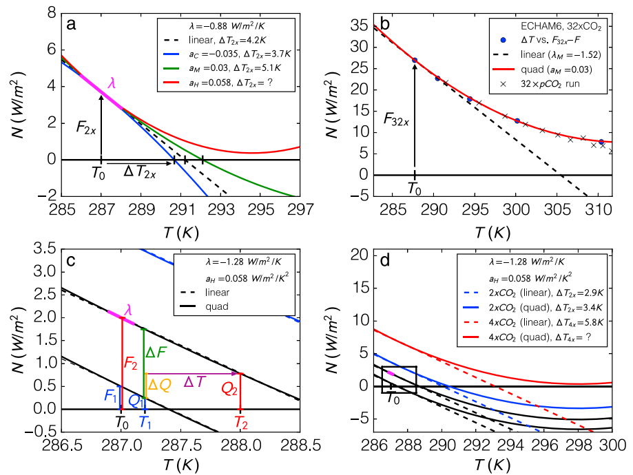
Figure 1. Global annual mean net top-of-atmosphere energy flux N (downward positive) as a function of global annual mean surface temperature T , where each curve has a fixed \text{CO}_2 concentration. (a) Doubling \text{CO}_2 increases N by a forcing F_{2x} \approx 3.71 \text{ W/m}^2 [Collins et al. , 2013]. All four curves have the same preindustrial feedback, \lambda (the slope of N at T_0 ), but different values for the feedback temperature dependence, a , resulting in different warming responses \Delta T_{2x} . Colored lines have values of a where the subscripts correspond to GCMs in Figure 2. For a_H (red curve), the feedback becomes positive, causing runaway warming. (b) ECHAM6 under five \text{CO}_2 doublings. We quadratically fit N to preindustrial conditions and the equilibrium response to four \text{CO}_2 forcings (blue circles [Meraner et al. , 2013]), adding F_{32x} to estimate N(T, 32C_0) (red curve). The time series of T versus N from the 32x\text{CO}_2 run (black crosses) follows this curve, until the model “blows up” (data from T. Mauritsen, personal communication, 2015). (c) Illustrative scenario with fixed values \lambda and a , showing how \lambda can be estimated from observations of surface temperature ( T ), forcing ( F ), and heat uptake ( Q ) from times 1 and 2. Warming appears linear. (d) Same scenario after one (blue) and two (red) \text{CO}_2 doublings, with the previous panel inset. The linear approximation works for one doubling, but under two doublings, the quadratic model runs away.
