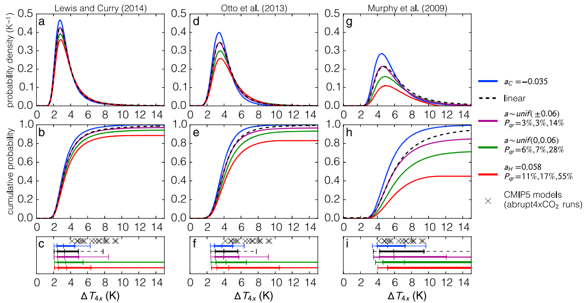
Figure 3. Distributions of \Delta T_{4x} recalculated from three observational studies to account for feedback temperature dependence. Linear distributions (dashed black lines) assume a constant feedback, recreating the results from the three studies, while the nonlinear distributions (colored lines) assume a has the minimum (blue lines) or maximum (red lines) value from our analyzed GCMs or assume a follows a uniform distribution covering the range \pm 0.06 \text{ W/m}^2/\text{K}^2 (purple lines) or 0 to 0.06 \text{ W/m}^2/\text{K}^2 (green lines). (a, d, and g) Probability density functions and (b, e, and h) cumulative density functions (CDFs) for these distributions. Distributions which allow for positive a (red, purple, and green lines) have a nonzero probability of quadratic runaway ( P_{qr} ), which causes CDFs to asymptote to values less than 1. These probabilities are listed for each distribution in the legend, with the values for the three studies separated by commas. (c, f, and i) Uncertainty ranges, where ticks demarcate 5th-17th-50th-83rd-95th percentiles, as compared with results from the CMIP5 abrupt4xCO 2 experiment (black crosses).
