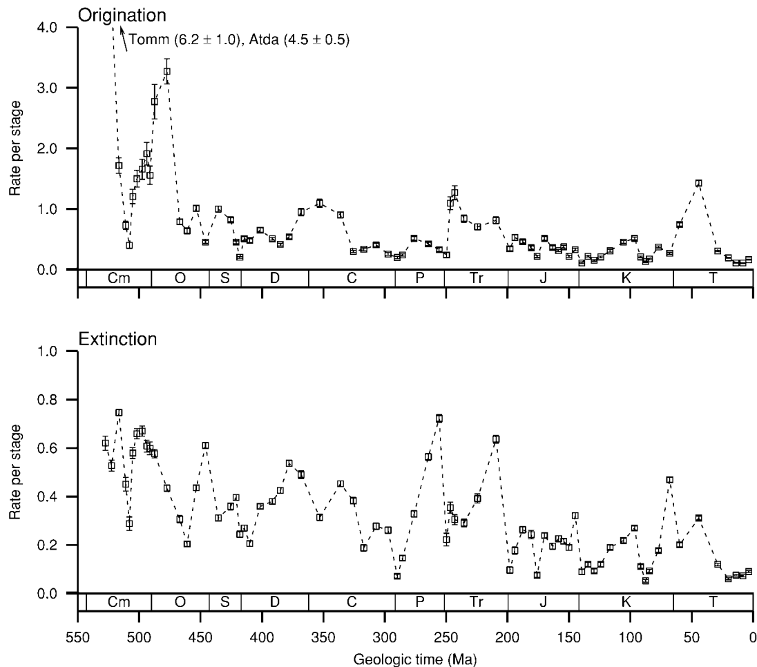
Figure 2. Observed rates of origination and extinction on the basis of the pulsed turnover model, with all originations and extinctions assumed to occur at stage beginnings and ends, respectively. Origination rate is equal to number of new genera in interval divided by number at start of interval, i.e., (X_{FL} + X_{Ft})/(X_{bL} + X_{bt}) . Extinction rate is equal to number of genera last appearing in interval divided by total interval diversity, i.e., (X_{FL} + X_{bL})/(X_{FL} + X_{bL} + X_{Ft} + X_{bt}) . Compare with figure 1. As with figure 1, first and last appearances are accepted as proxies for origination and extinction events.
