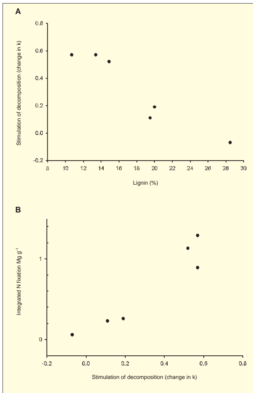
Figure 2. A. The relationship between lignin concentration (a measure of carbon quality) and the increase in decomposition rate caused by added N in Metrosideros polymorpha litter from Hawaii. From Hobbie (63, 65).
