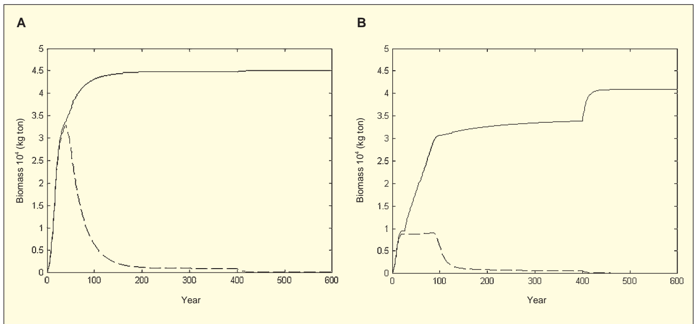
Figure 1. Simulated effects of constraints to symbiotic N fixation on total plant biomass (solid line) and the biomass of N fixers (dashed line). A. Biomass assuming that symbiotic N fixation involves a substantial energy cost, but no additional constraints. B. Biomass assuming that symbiotic N fixation is further constrained by differential shade intolerance, P limitation, and grazing. In both cases, a step increase in N additions occurs in year 400; the magnitude of response to that addition is a measure of N limitation. Based on analyses in Vitousek and Field (51).
