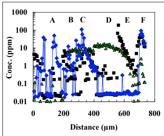
Figure 1: Traverse (12 \mu\text{m} beam diameter, 4 \mu\text{m/s} ) across the palisade body in GBS from Allende (Hf: green triangles, W: black squares, Pt: blue diamond).
